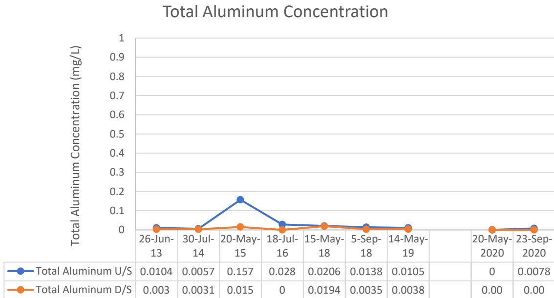
Figure 5. Total aluminum concentration over time.
