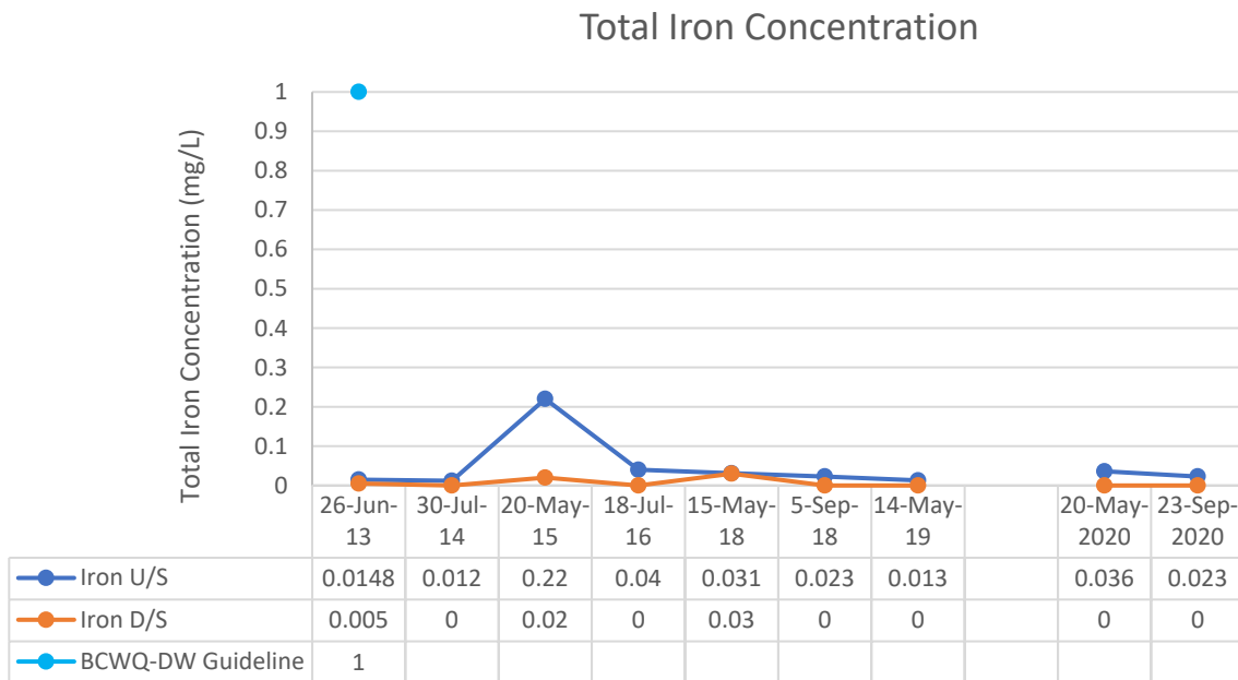
Figure 6. Total iron concentration over time.
